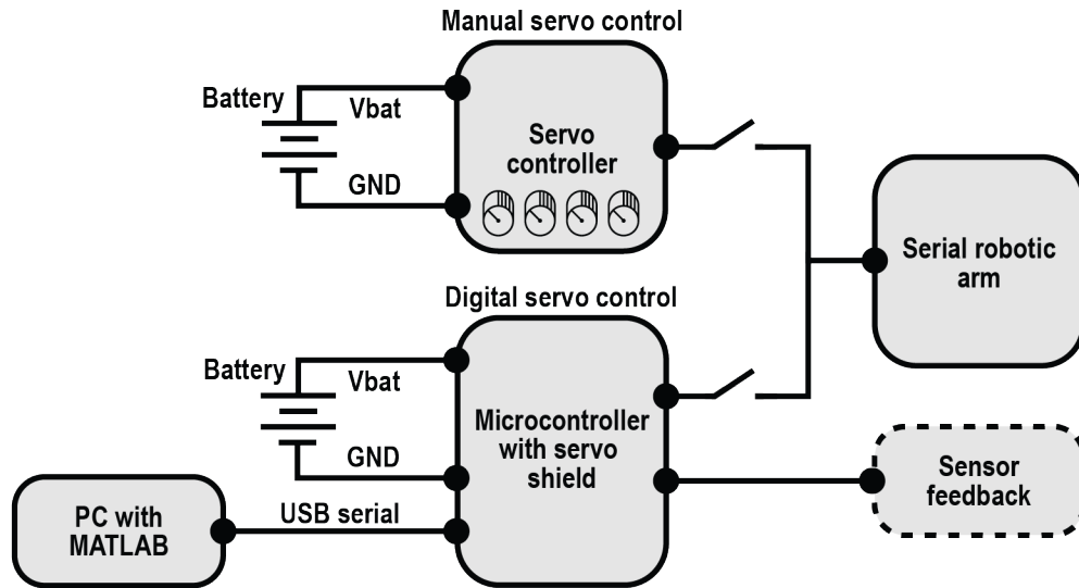
Figure 2: Schematic illustration of the robotic arm kit. The serial robotic arm can be manually controlled using a servo controller or digitally controlled using a microcontroller via a servo shield. Commands can be generated directly from the microcontroller, or a computer equipped with MATLAB or other software. The kit was powered using a laptop computer or USB battery pack to allow for untethered use in a classroom or general study environment.
