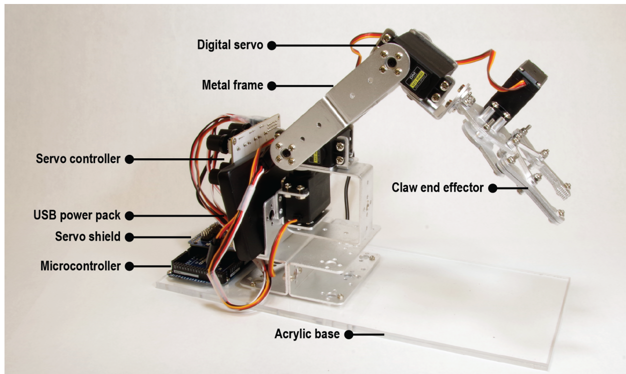
Figure 1: Photograph of the robotic arm kit with control electronics and power pack for untethered use in a classroom or general study environment.
