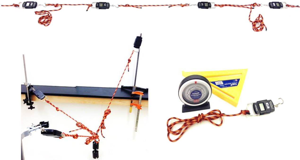
Figure 1. Force equilibrium activities: (Top) 1-D Equilibrium “Tug of War”, (Bottom Left) 3-D Equilibrium, (Bottom Right) Force & Angle Measurement Devices
