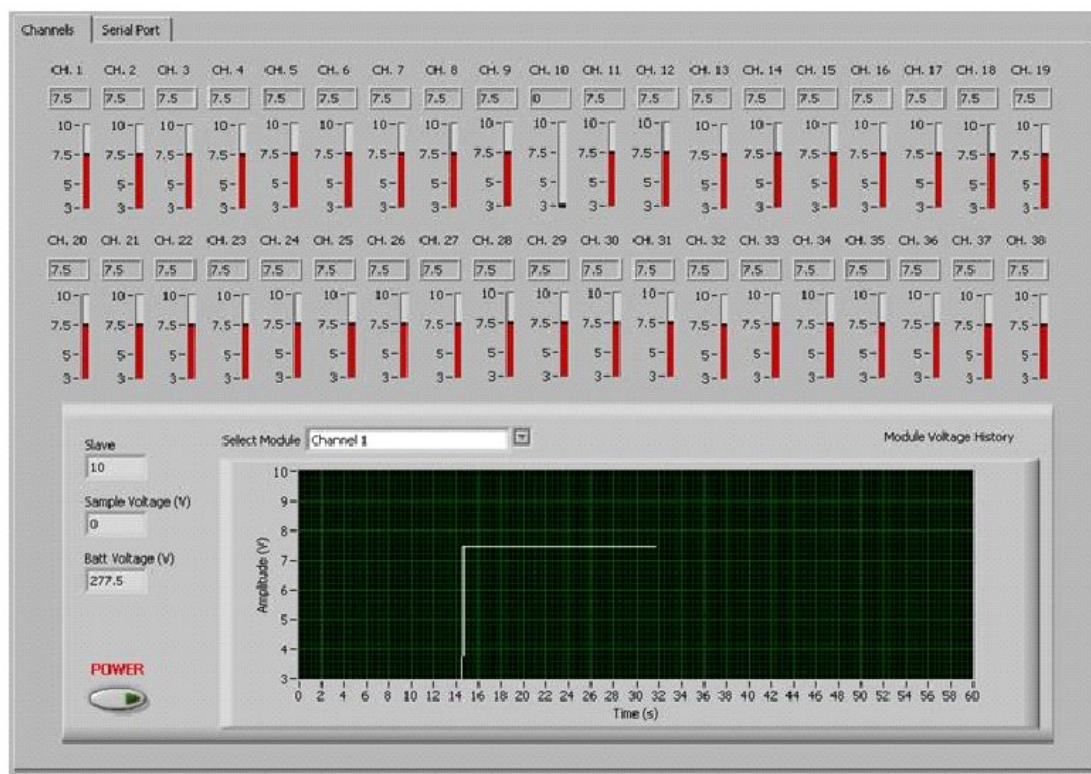
Figure 9. Battery Monitoring System LabVIEW Display 15
