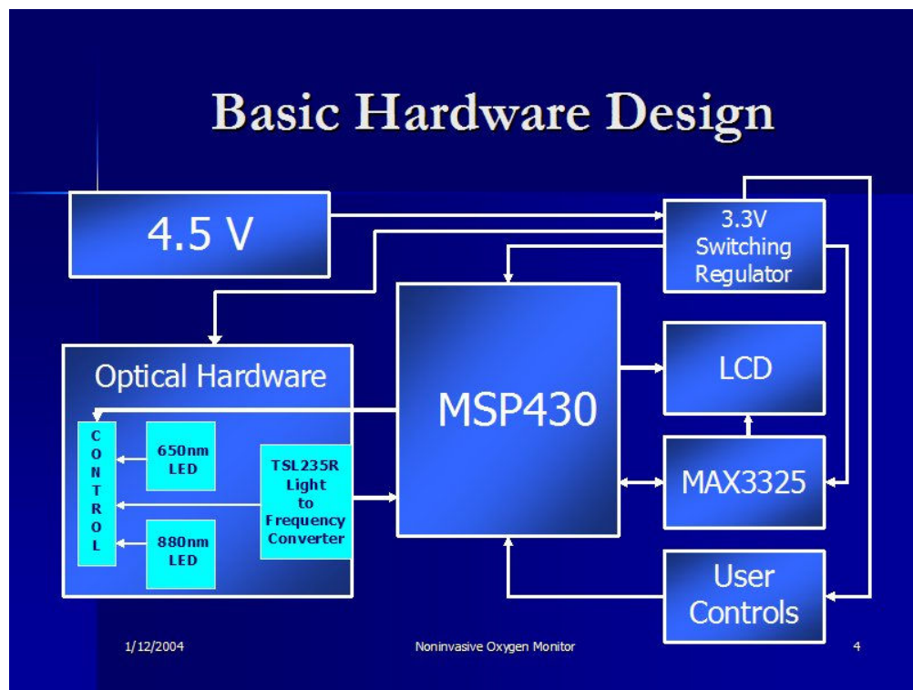
Figure 5. Blood Oxygen Monitor Block Diagram 13
