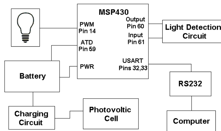
Figure 1. Remote Lighting Block Diagram 12
