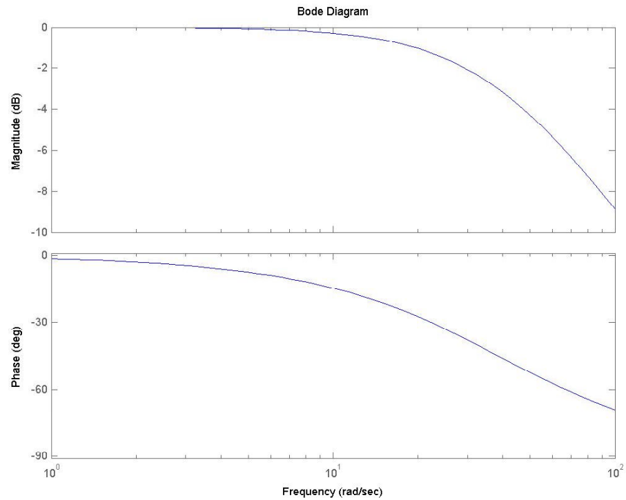
Bode Plot
