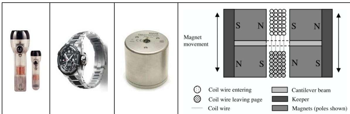
Figure 7. Examples of inductive vibration harvesters: (From left to right) Faraday flashlights 35 , Seiko Kinetic Drive watch 36 , Perpetuum PMG37 micro-generator 37 , schematic of the University of Southampton research harvester 38 .
