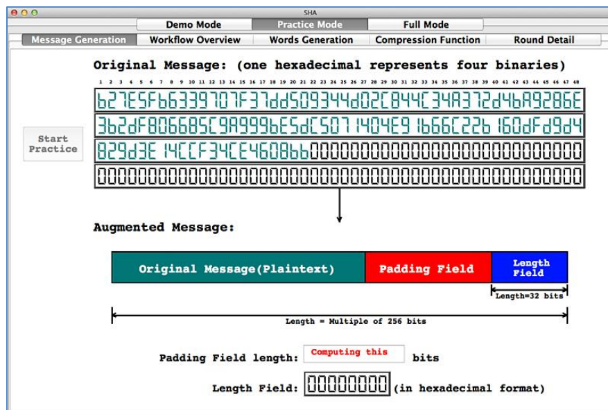
Figure 7: Practice Mode of SHAvisual
