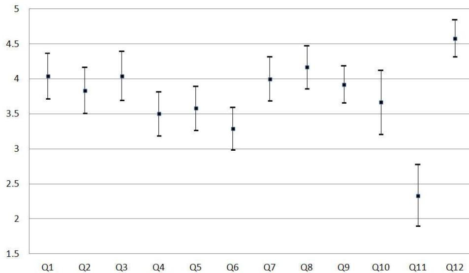
Figure 10: Interval Plot of Table 2
