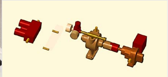
Figure 2: CREO Parametric Simulated 3D Model of the Apparatus
