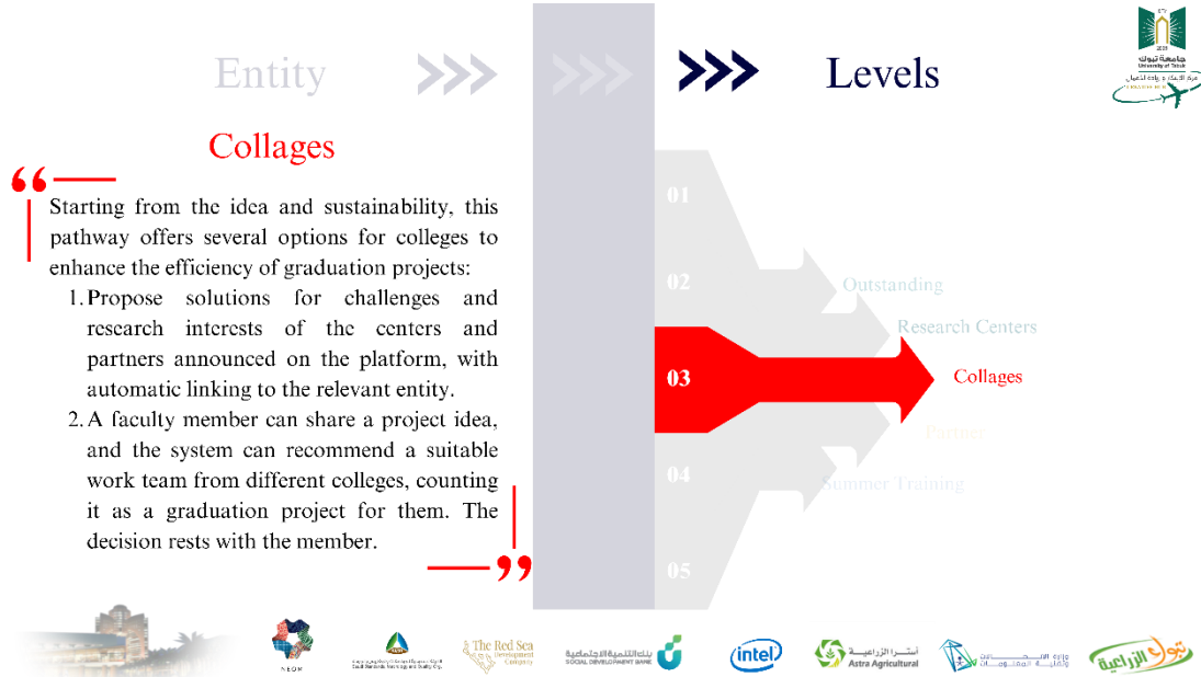
Figure 6: Collages Path
