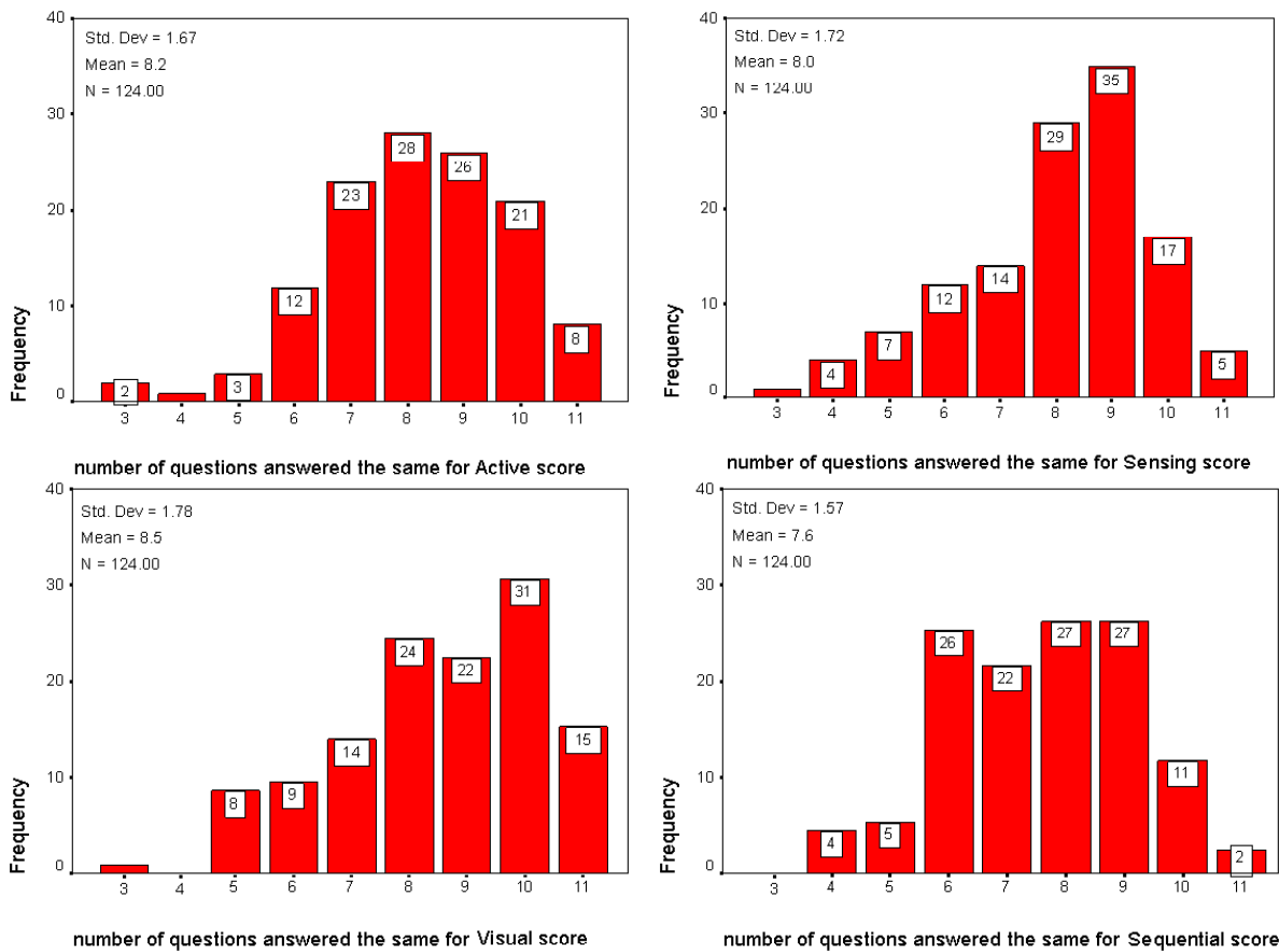
Figure 1: Histogram of Identical Responses to Items on Test-Retest
