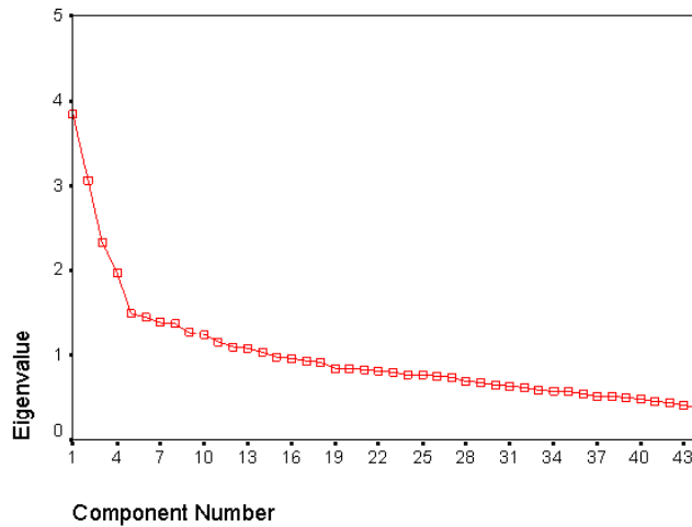
Figure 2: Scree Plot for Factor Analysis on ILS Scores (n = 551)
