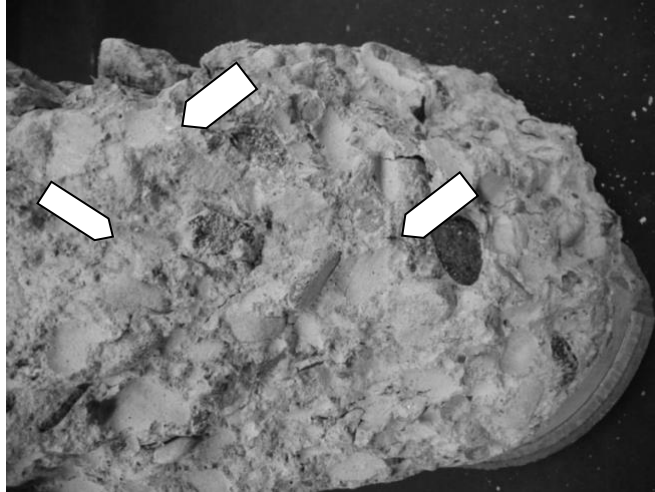
Figure 6. Aggregate fracture in cylinder with low water-to-cement ratio mix
