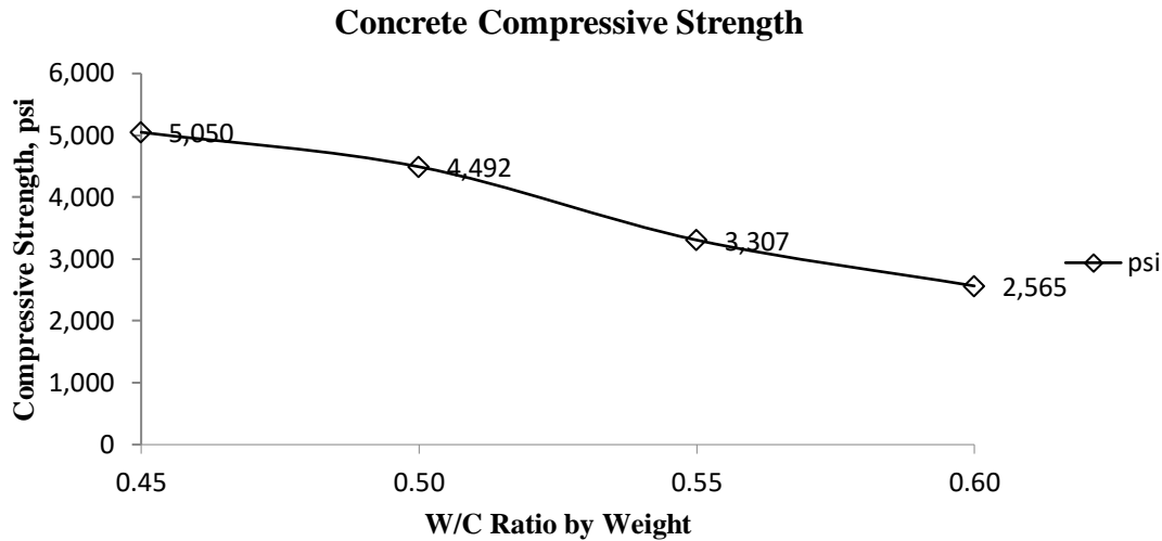
Figure 7. Compressive strength graph by water cement ratio
