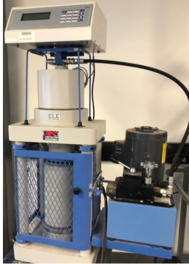
Figure 5. Digital Concrete compression tester with readout
