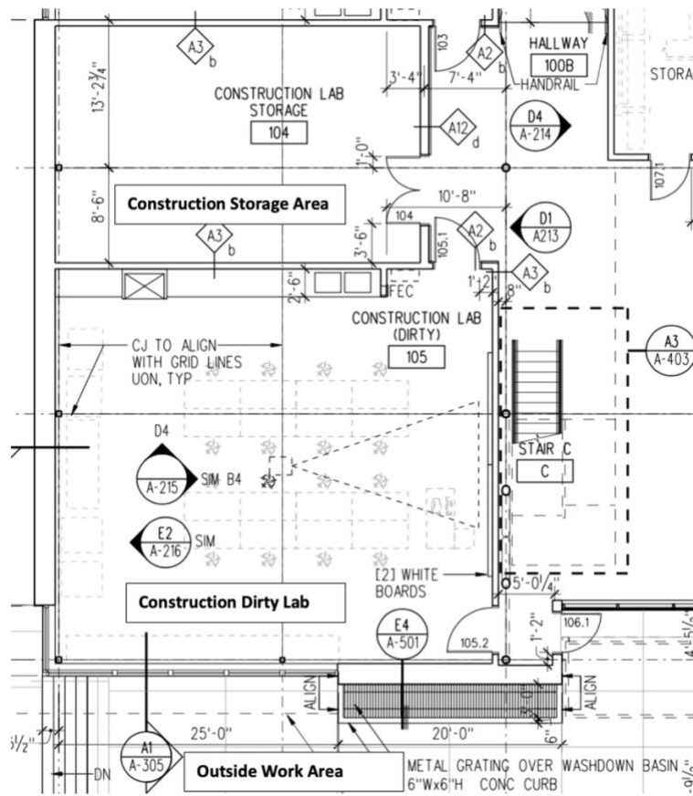
Figure 1. Hogue Hall Lab, Storage, and Outside Work Area Layout
