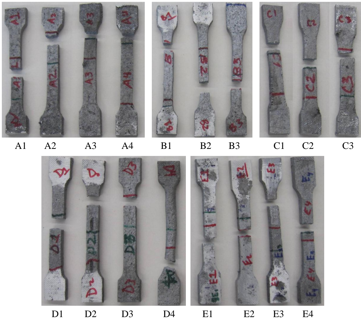
Figure 8: Broken specimens with the potential critical cross sections marked by students. Their predictions were confirmed for specimens A3, B3, C2, D3, E2, E4. Specimen D4 failed prematurely because of a gross inclusion.
