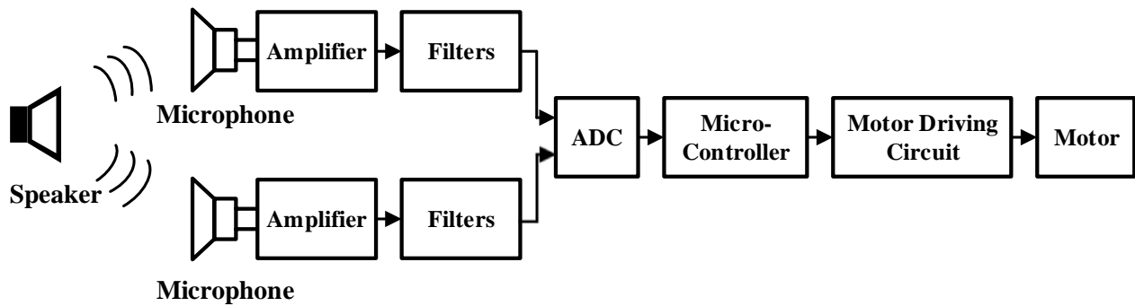
Figure 2: System diagram of the sound-following robot
