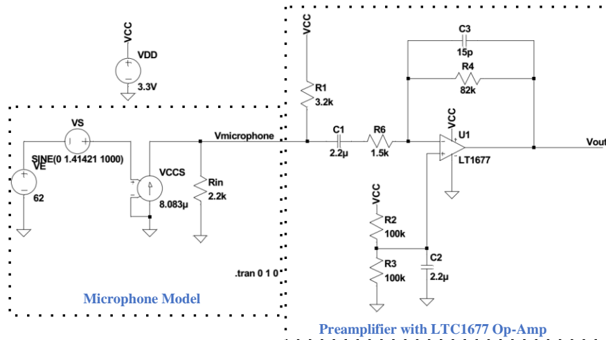
Figure 6: The schematic of the audio amplifier circuit in LTSpice
