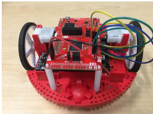
Figure 8: TI RSLK with TI MSP430 microcontroller, DC motor and driving board
