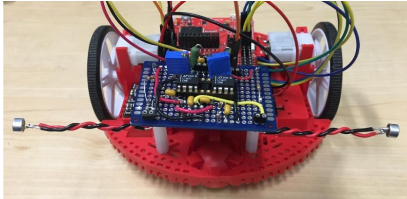
Figure 1: Music-following robot using TI RSLK kit
