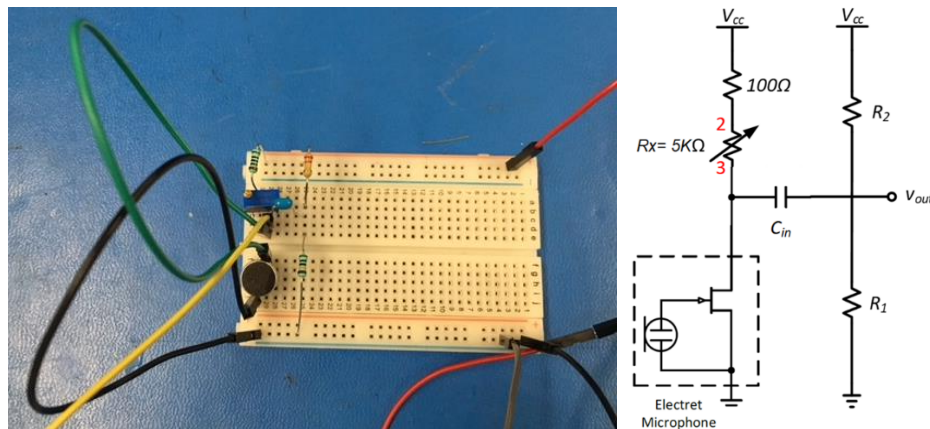
Figure 3: Microphone bias circuit on breadboard.
