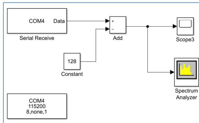
Figure 7: Using MATLAB and UART communication for plotting the frequency spectrum of audio signals
