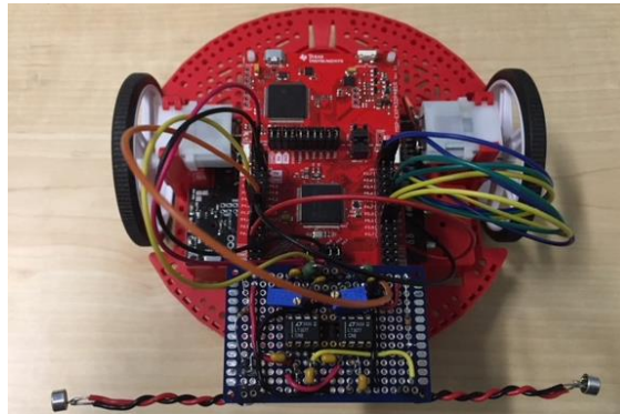
Figure 9: Completed music-following robot
