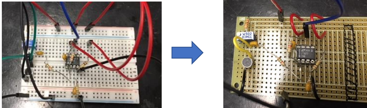
Figure 5: Sound detecting circuit on a breadboard and a prototype board
