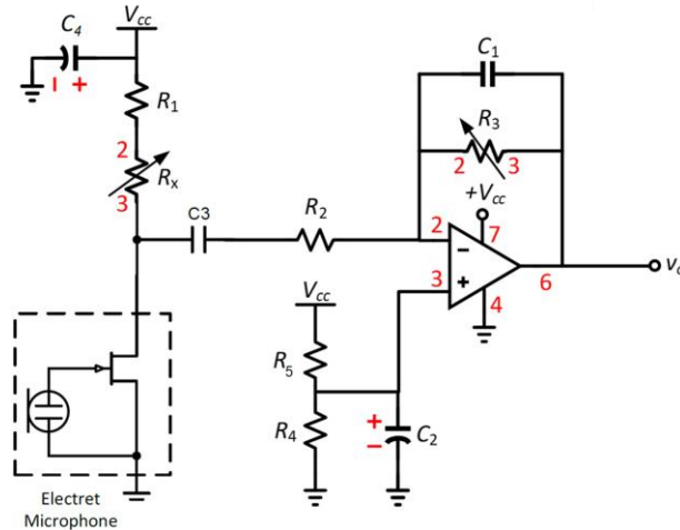
Figure 4: Filter and amplifier for the sound detecting system
