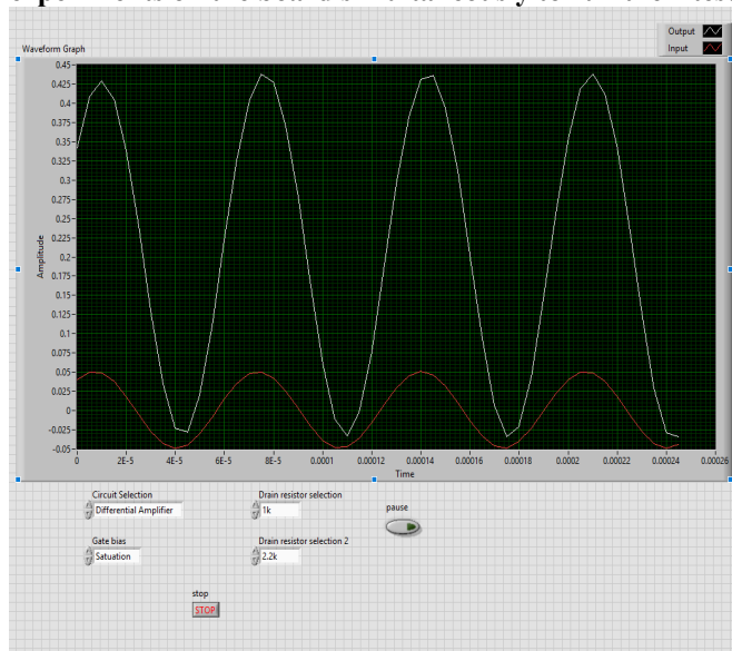
Fig. 2 Graphical user interface.
