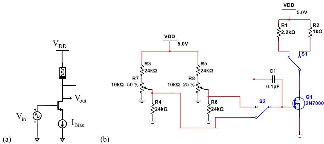
Fig. 5 Schematic of, (a) common source amplifier; (b) proposed reconfigurable common source amplifier with tunable loads and current biasing implemented using potentiometers. The small signal input is applied through capacitor C1. The analog switches (S1 and S2) are also shown that the students will configure remotely.
