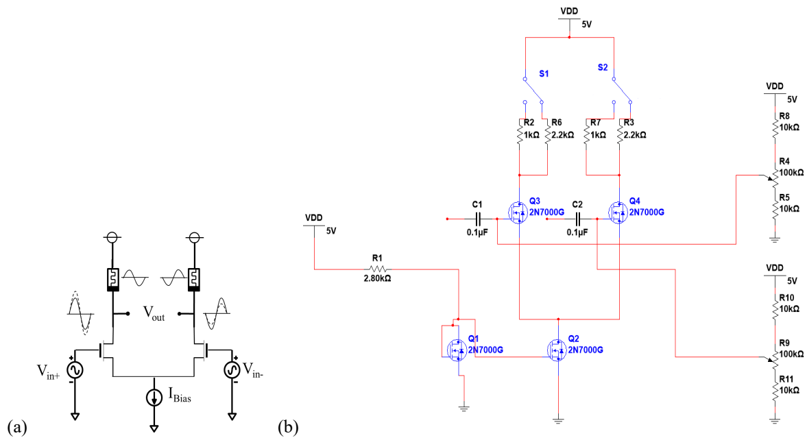
Fig. 6 Schematic of, (a) differential amplifier; (b) proposed reconfigurable differential amplifier with tunable loads and current biasing. The small signal input is applied through capacitor C1 and C2. The analog switches (S1 and S2) are also shown that the students will configure remotely.
