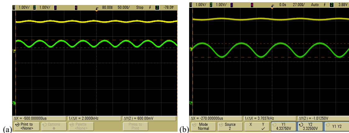
Fig. 7 Common source amplifier working in saturation region with, (a) 1\text{K}\Omega load resistor using switch S1 and, (b) 2.2\text{K}\Omega load resistor using switch S2. The yellow waveform is small signal input whereas green waveform is the amplifier output.
