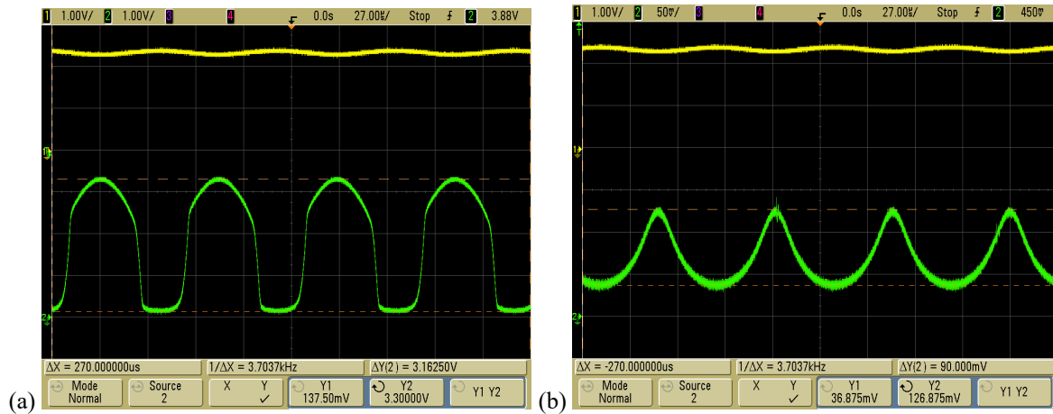
Fig. 8 Common source amplifier working in linear region with, (a) 1K \Omega load resistor using switch S1 and, (b) 2.2K \Omega load resistor using switch S2. The yellow waveform is small signal input whereas green waveform is the amplifier output.
