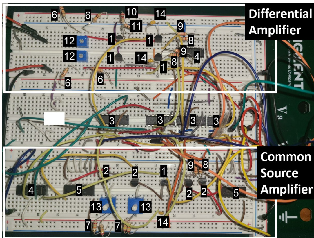
Fig. 3 Physical layout of the board. Various components from Table-1 have also been labeled.
