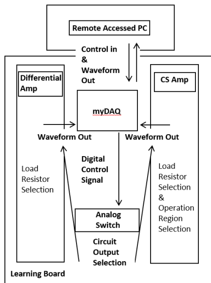
Fig. 4 A High-level diagram of the connections and signal flow of the components. The myDAQ is the element that translates the control signal from PC to hardware elements and send the signal readout to the graphical user interface. The analog switch is used to select the proper waveform as output following the control signal from myDAQ.
