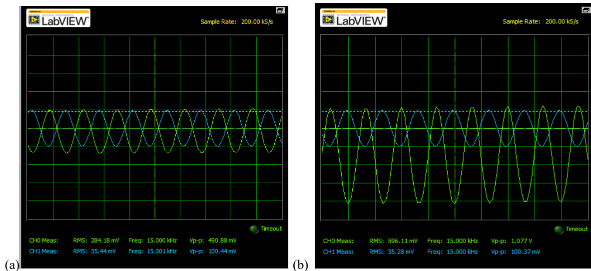
Fig. 9 Differential amplifier working in saturation region with, (a) 1K \Omega load resistor using switch S1 and, (b) 2.2K \Omega load resistor using switch S2. Blue is the input and green is the output waveform.
