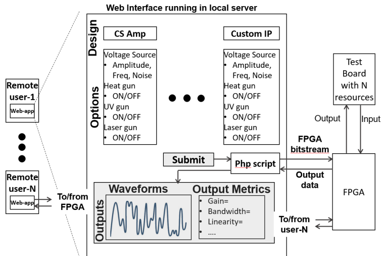
Fig. 1 Overview of our approach. The student will select the design for experimentation (or write a netlist) and enter the options. After submitting the request, a php script will compile the user selections to FPGA bitstream which in turn will apply the settings on the board using available resources. The sampled output from test board is collected by the FPGA and sent back. Multiple students will be able to execute experiments on the board simultaneously to run their test cases independently.
