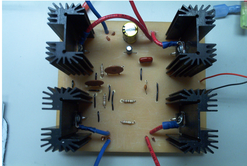
Figure 8. MOSFET
