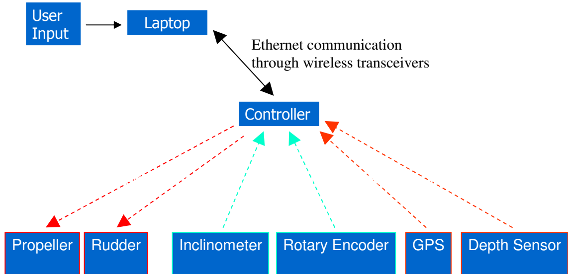
Figure 4. Flow of data and control signals
