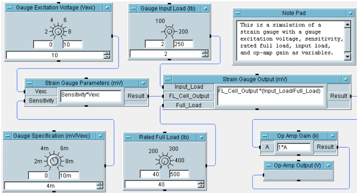
Figure 3 Program for Strain Gage Simulation with Open Icons
