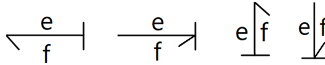
Figure 1: Possible orientations of flow direction (half-arrow) and causal stroke (represented by the horizontal line perpendicular to the bond).
