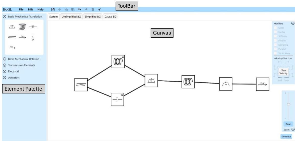
Figure 6: Screenshot of the bond graph software shown with a mechanical system and annotations for key features such as Canvas, Element Palette and ToolBar.
