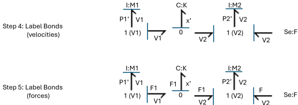
Figure 3: Assignment of effort and flow variables.
