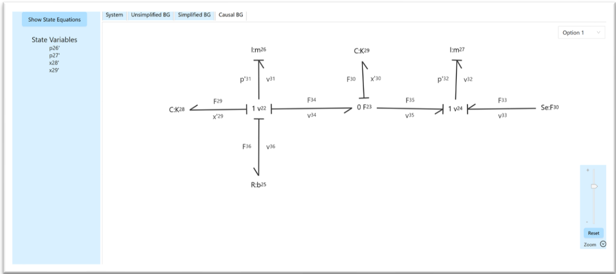
Figure 12: Screenshot of the causal bond graph generated by the program with state variables displayed on the left panel.
