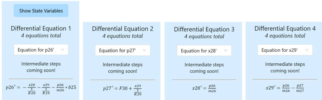
Figure 13: Screenshot of the four state equations generated by the bond graph program.
