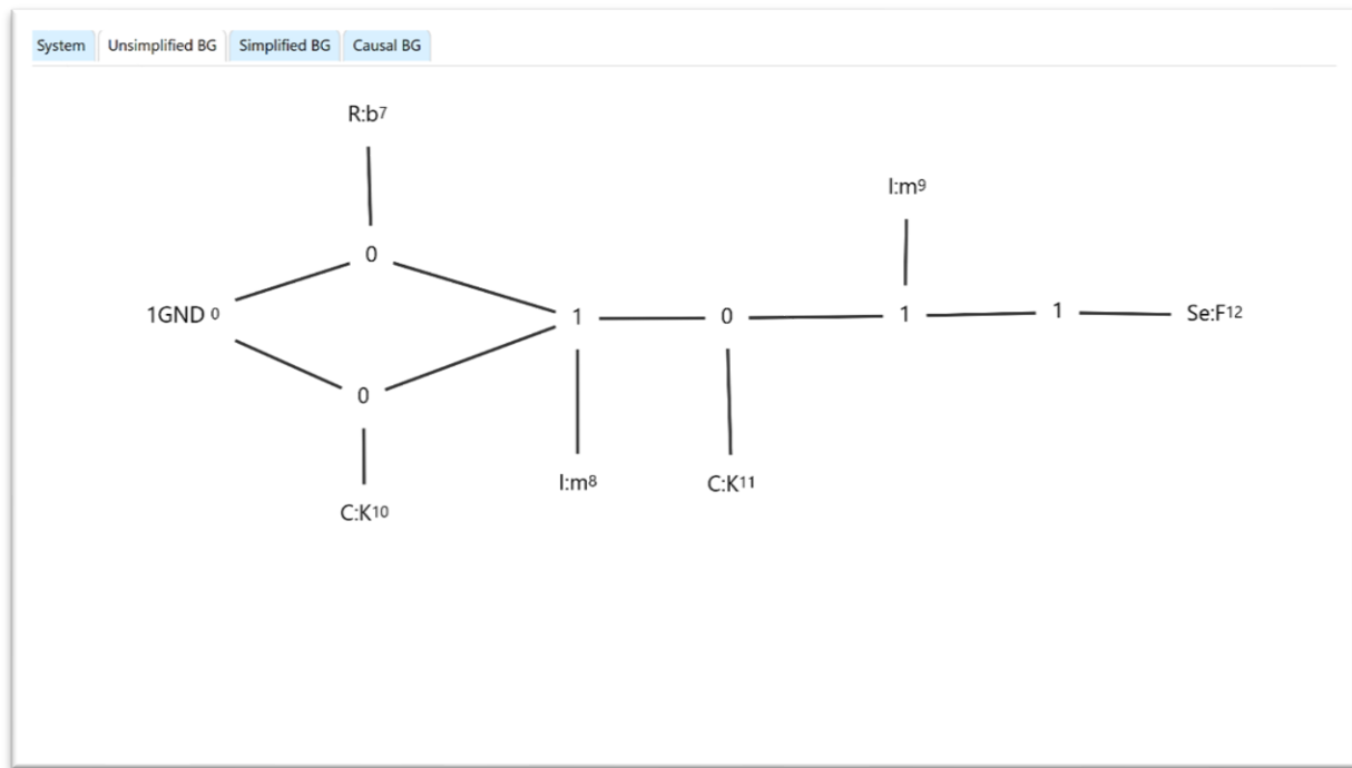
Figure 10: Screenshot of the Unsimplified bond graph that has been manually reorganized.
