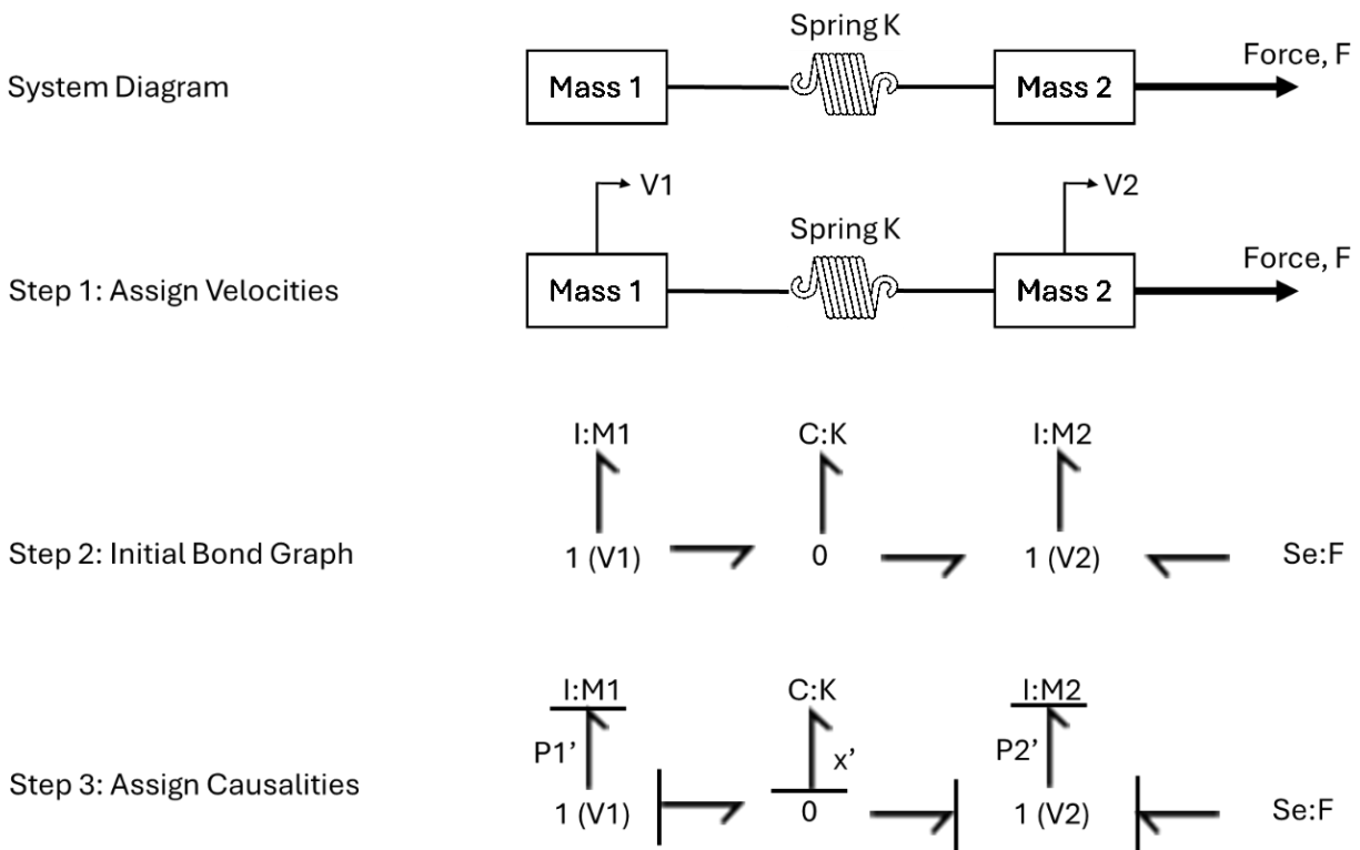
Figure 2: Derivation of causal bond graph from system diagram.
