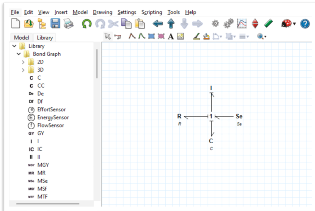
Figure 5: A bond graph as displayed in the 20-sim interface.
