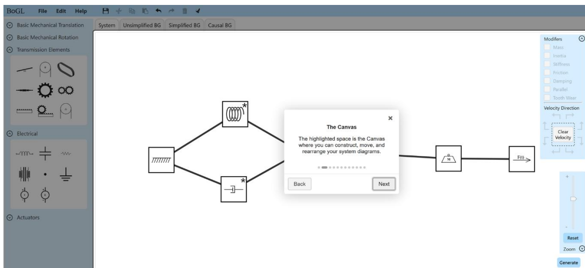
Figure 8: Screenshot of the interactive tutorial within the application.
