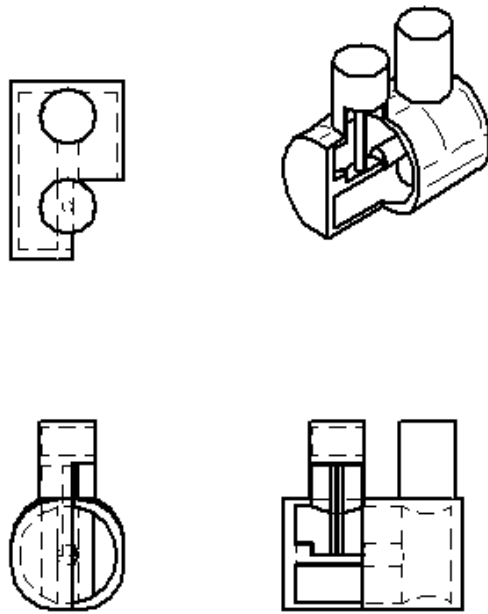
Figure 3: Orthographical view of motor driven engine
