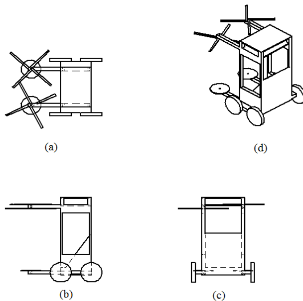
Figure 2: Orthographical views of concept robot (a) top view (b) right side view (c) front side view (d) complete view
