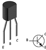
Figure 4. Transistor.
