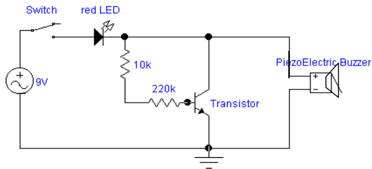
Figure 6. The Doorbell Electric Circuit.
