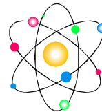
Figure 1. An atom.
