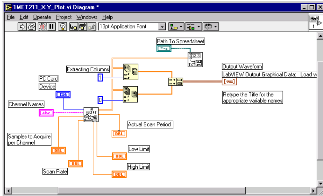
Figure 4: LabVIEW™ VI Diagram for Load vs. Deflection Plot
