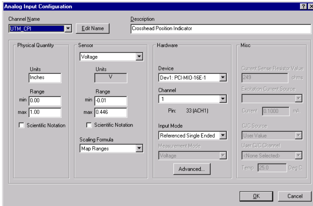
Figure 7: LabVIEW™ Analog Input Configuration for the UTM Crosshead Position Indicator
