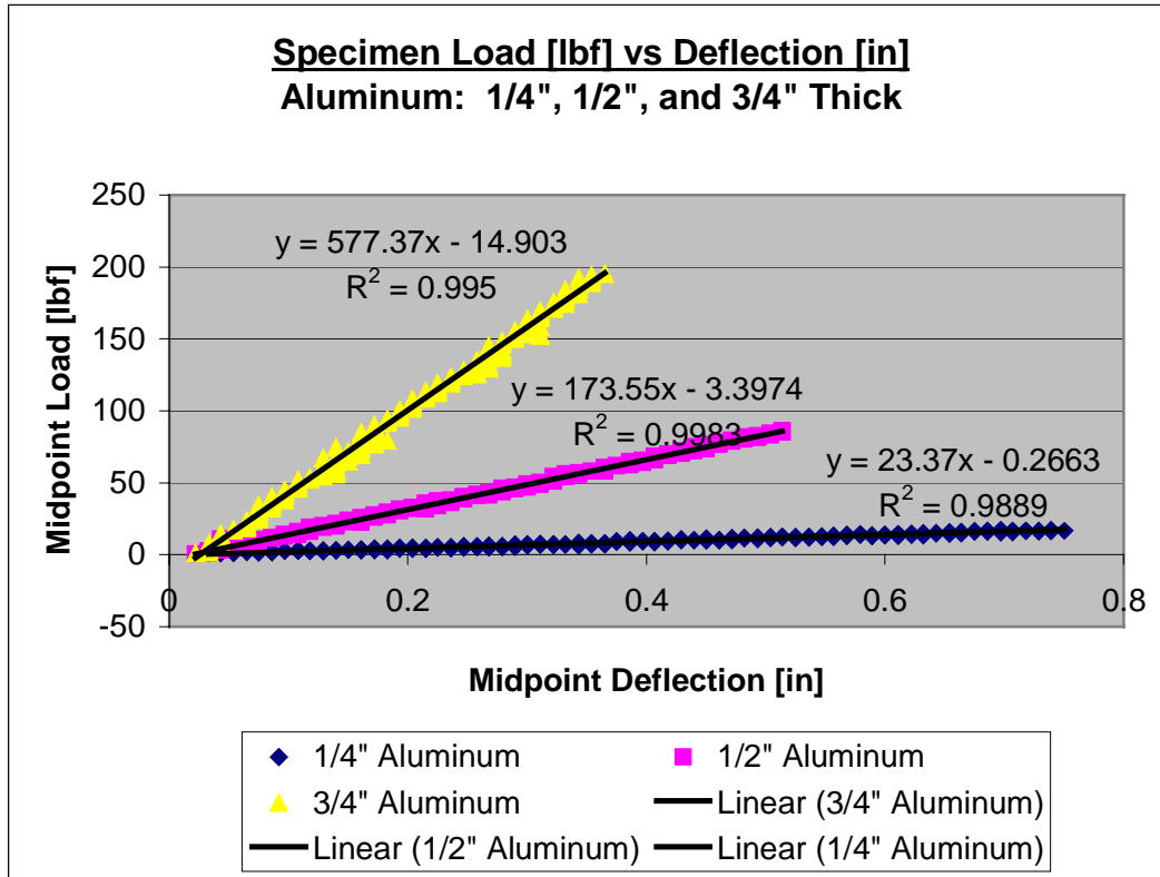
Figure 3: Raw Test Data Acquired During Test Plotted in Excel™ Spreadsheet with Regression Lines
