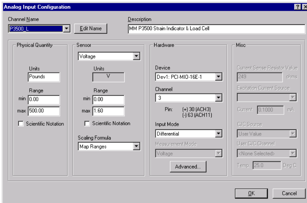
Figure 6: LabVIEW™ Analog Input Configuration for the UTM Load Cell
