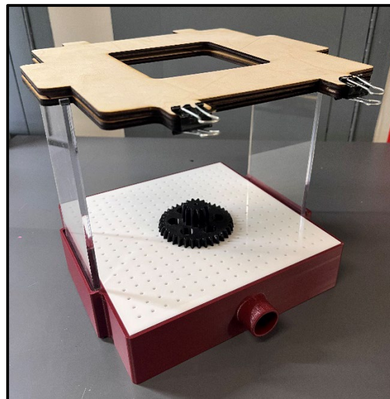
Figure 2.10. Final Device
