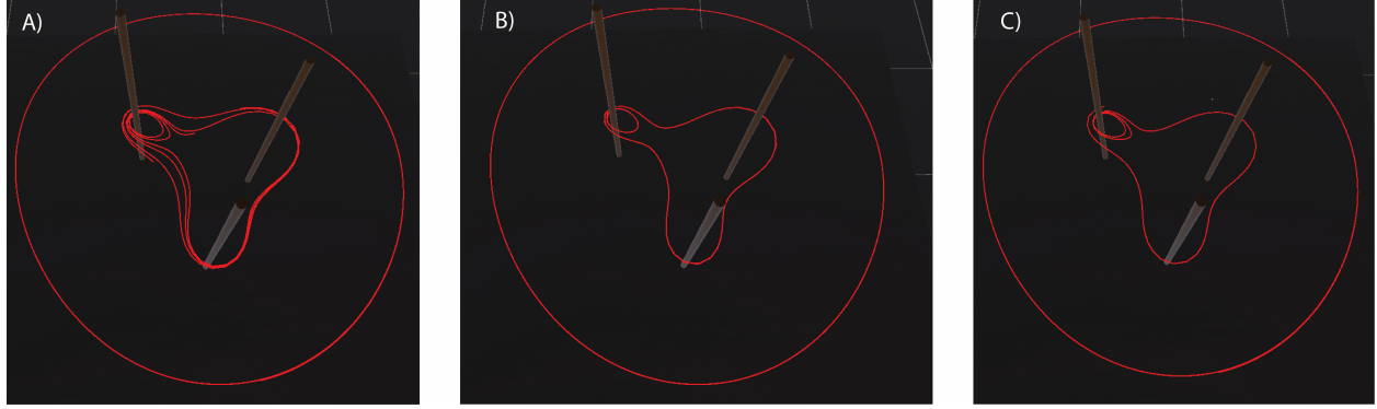
Figure 1: A system of three infinite wires generating a magnetic field. Three field lines are traced using A) Euler Forward, B) Heun's method, and C) RK4
