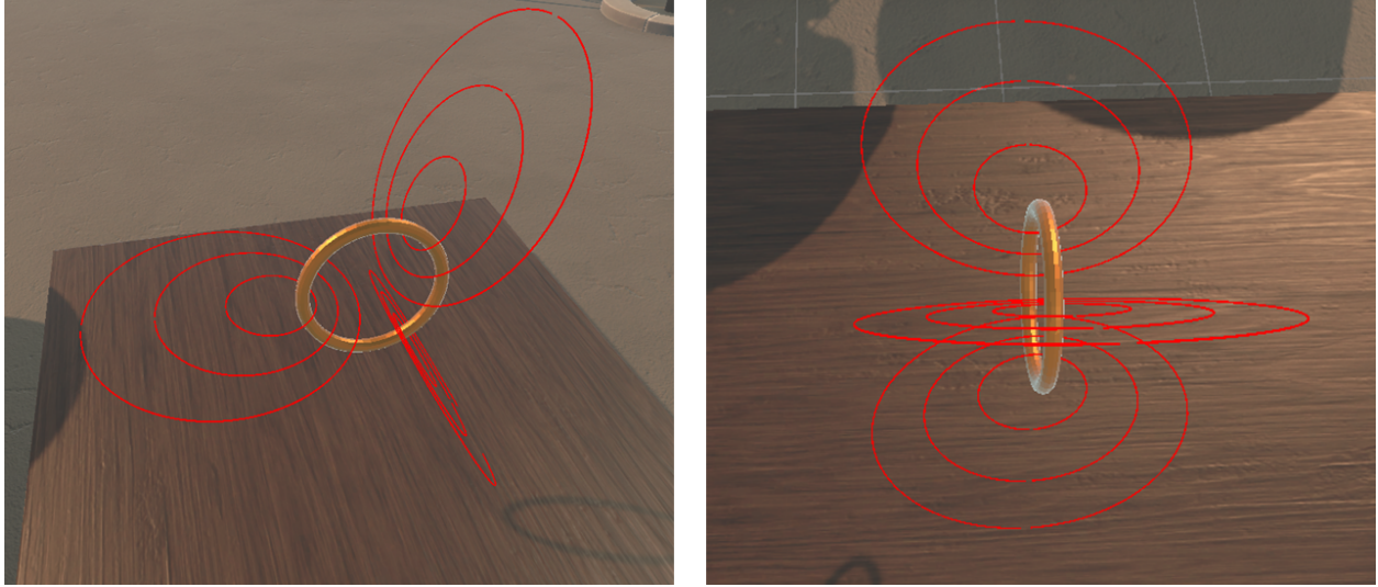
Figure 2: Magnetic field lines generated from a current-carrying loop approximated with ellipses.
