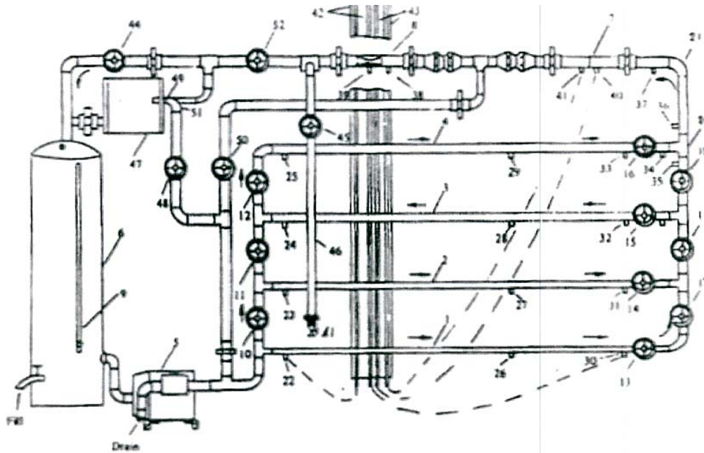
Figure 1: Piping System Diagram
