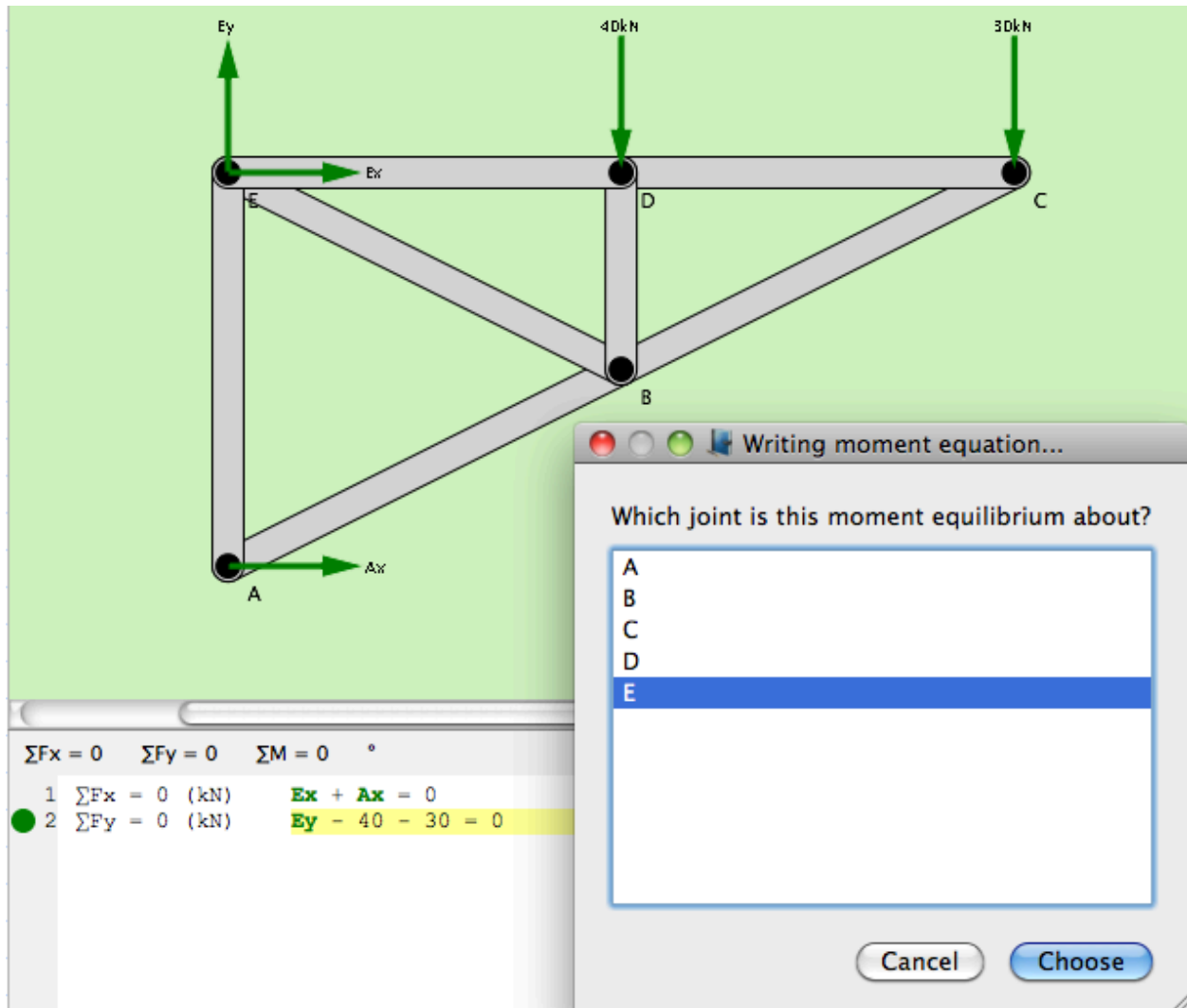
Figure 4. Screen shot of writing equations, and choosing moment center.
