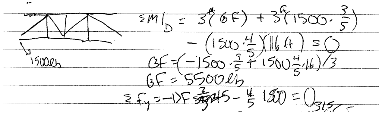
Figure 1. Example of typical student error: Internal forces (GF and DF) are not drawn on section, but appear in equilibrium equations; the solutions ultimately have sign errors.
