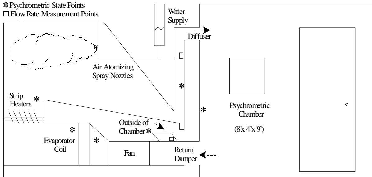
Figure 1. Psychrometric Chamber Layout
