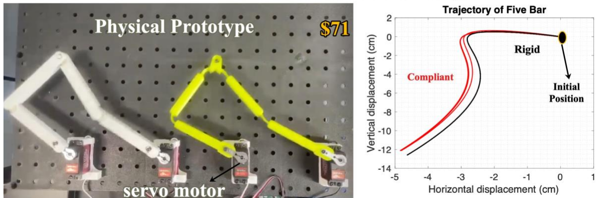
Figure 9. Simulation of compliant and rigid five-bar mechanisms
