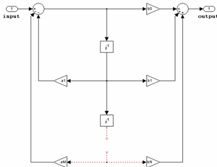
Figure 2: Generalized Direct Form II IIR Structure
