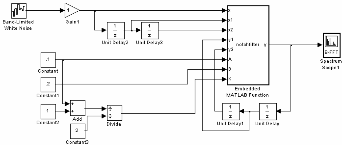
Figure 1: Simulink Notch Filter
