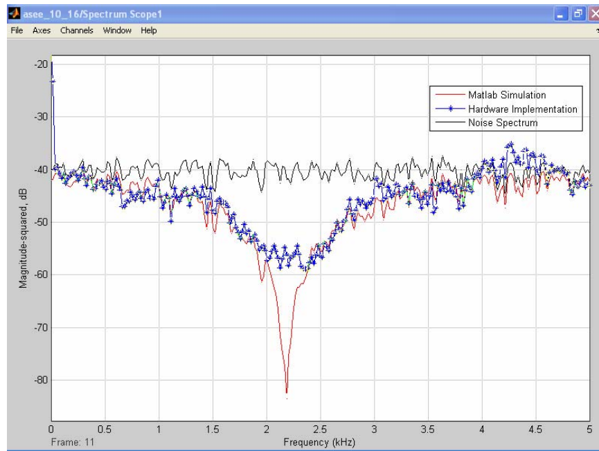
Figure 7: Filter Output Spectrum (8-bit word)
