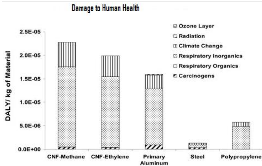
Figure 6: Vapor-grown carbon nanofibers life cycle assessment (VGCNF-LCA): damage indicators (disability-adjusted life years) [13].
