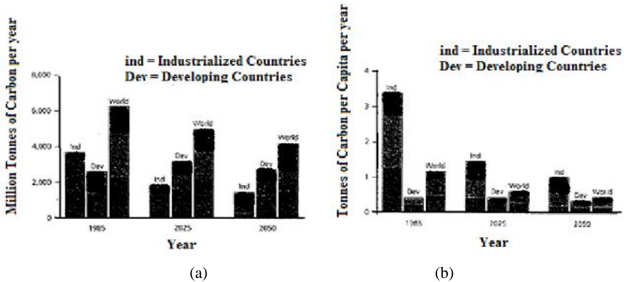
Figure 3: (a) Emissions of carbon dioxide for renewable intensive global scenario; (b) per capita emissions of carbon dioxide for renewable intensive global energy scenario [11].
