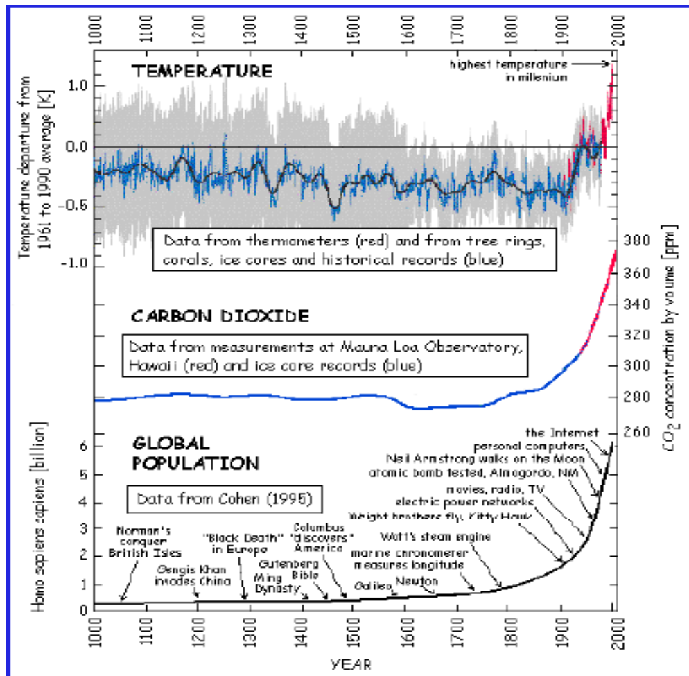
Figure 2: Comparison of increases in temperature, carbon dioxide emissions, and world population from year 1000 to 2000 [5].
