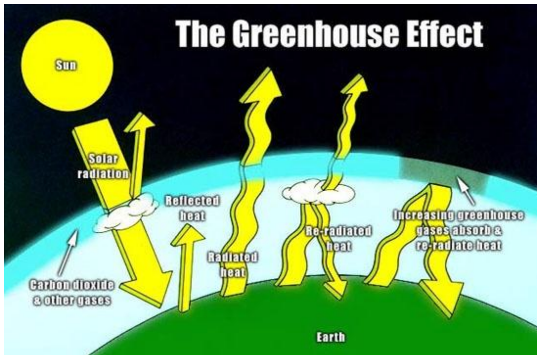
Figure 1: Greenhouse effect on the Earth's surface [4].
