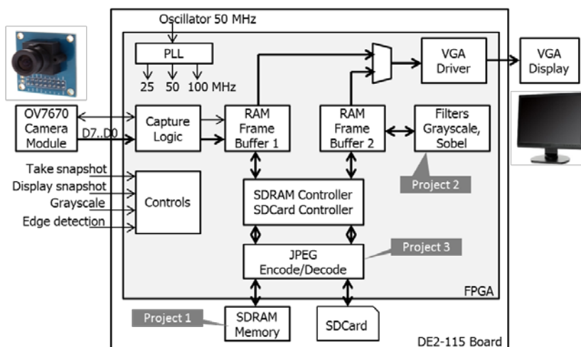
Figure 2: Top-level block diagram of the main product, a digital camera system, designed in this course.
