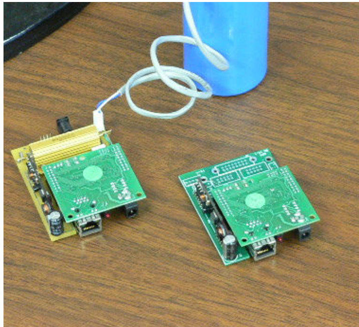
Figure 3. Two embedded Ethernet controllers with Power-Over-Ethernet (POE) capability, for reporting power statistics for the roof-top PV and turbine.
