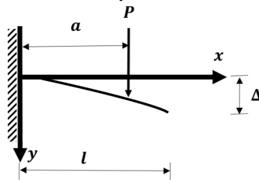
Figure 3. Cantilever steel beam with a point load varying along the length
