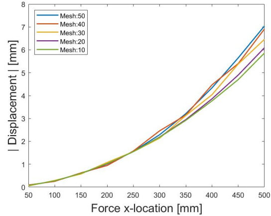
Figure 5. 2D plot on beam deflection under point loads with different mesh sizes
