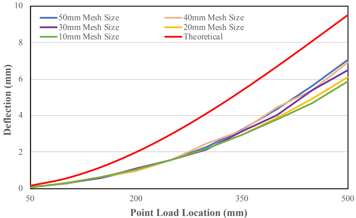
Figure 6. Comparison between numerical and theoretical values
