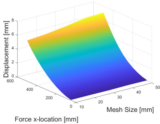
Figure 4. 3D plot on beam deflection under point loads with different mesh sizes
