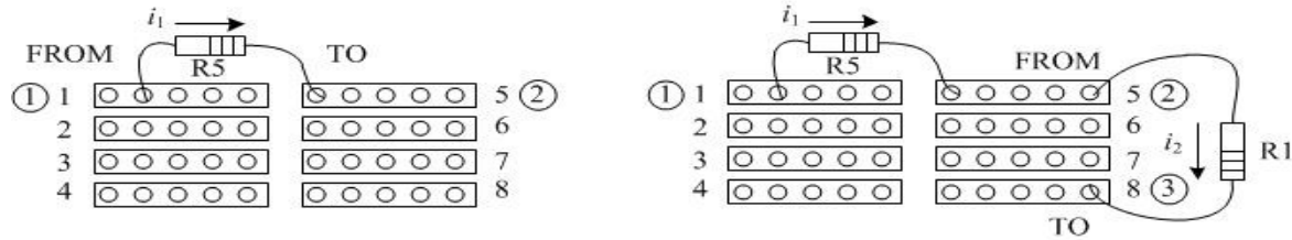
Fig 1: Depiction of virtual breadboard
