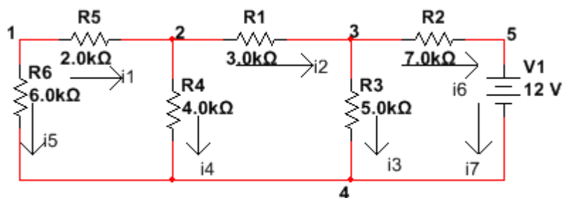
Fig 3: Circuit diagram of example circuit
