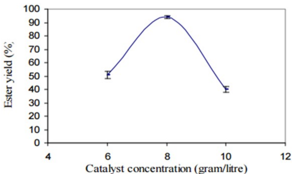
Figure 5: The conversion efficiency of ester under different catalysts concentrations [11].
