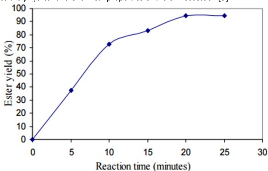
Figure 4: The graphic showing the trend of ester yield / conversion as a function of time [19].
