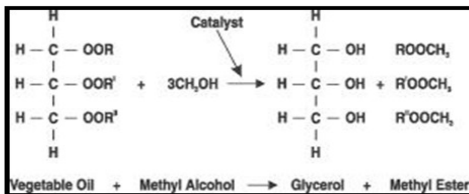
Figure 3: The transesterification process of converting vegetable oils into biodiesel (methyl ester) [14].
