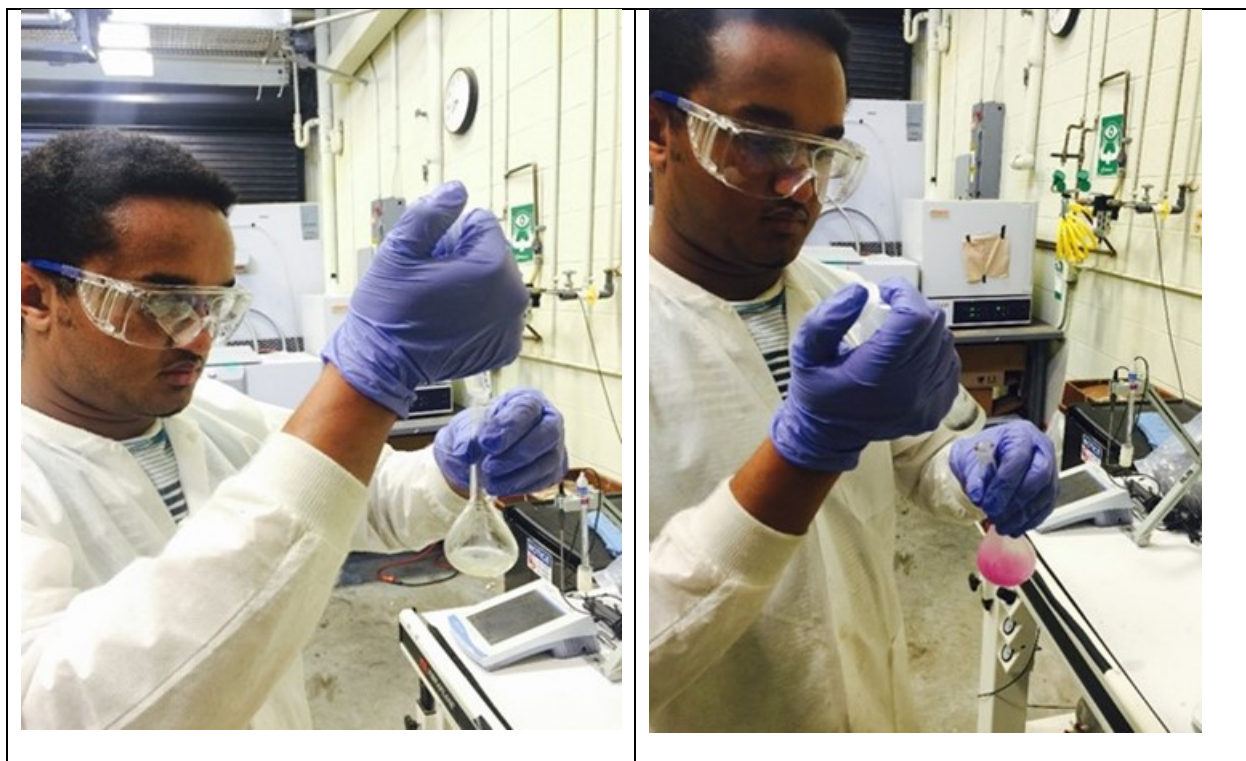
Figure 7: The titration process for the biodiesel production using the waste vegetable oil. The titration process was continued until the pink color was clearly seen.
