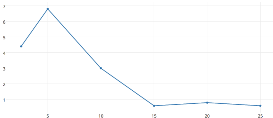
Figure 3. Plot of force required to balance a load vs. position of the effort from the fulcrum generated via plot.ly by a student group.
