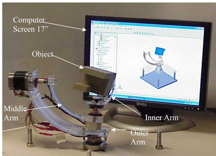
FIGURE 2 – PHYSICAL MODEL ROTATOR
