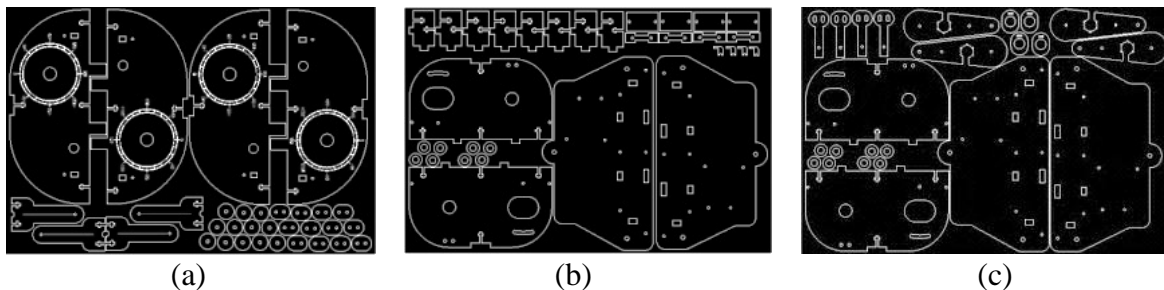
Figure 2. Haptic Paddle parts for four Paddles arranged on three 12''x18'' sheets, each containing: (a) Front plates, accessory washers, and handles. (b) Base and back plates, stabilizers, accessories. (c) Base and back plates, sensor board holders, motor mounts, and accessories.
