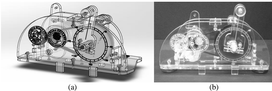
Figure 1. The Haptic Paddle design finalized by the Mechanical Engineering group. (a) SolidWorks model. (b) Manufactured unit.
