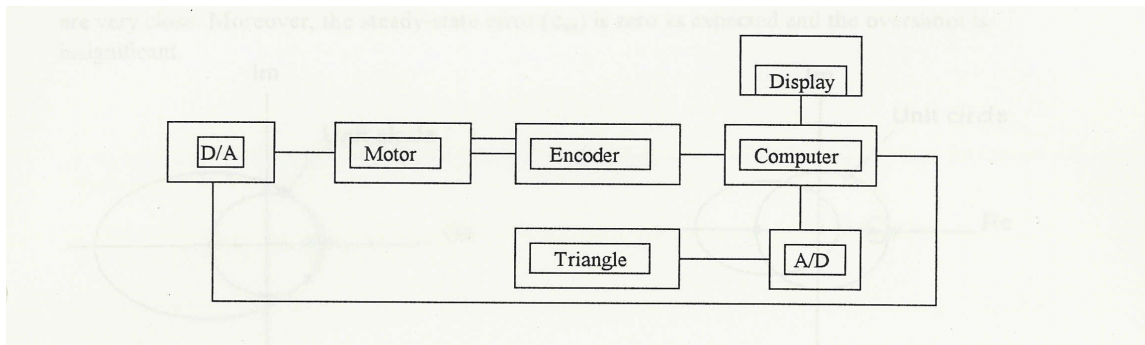
Figure 2. Block diagram of the SFT154 shaft encoder position control
