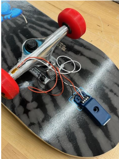
Figure 9– Strain Gage application for LabView Results of Aluminum Truck Deformation
