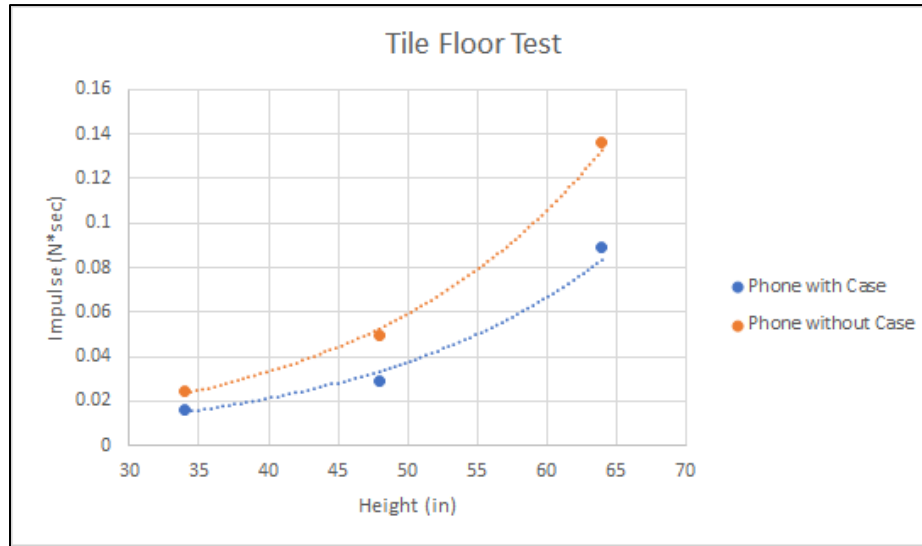
Figure 7: Comparison of impulse for the phone with and without the case over the tile floor. The phone did not receive any noticeable screen damage after both drop modes.
