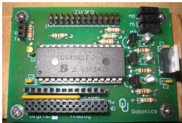
Figure 3: Multiplexer board used by AME 4802 students
