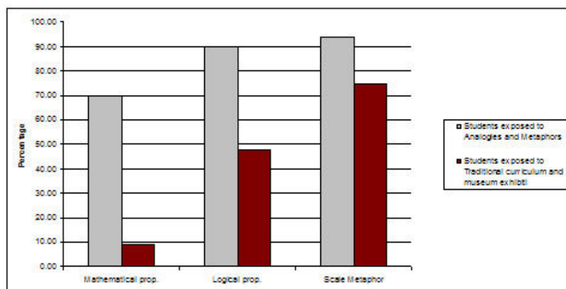
Figure 2. Summarized results
