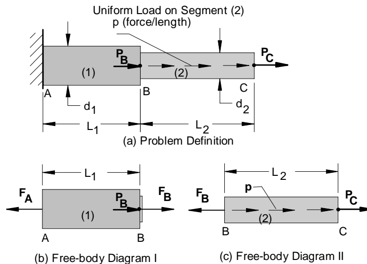
Figure 3. Two segment determinate bar problem with concentrated loads and distributed load.
