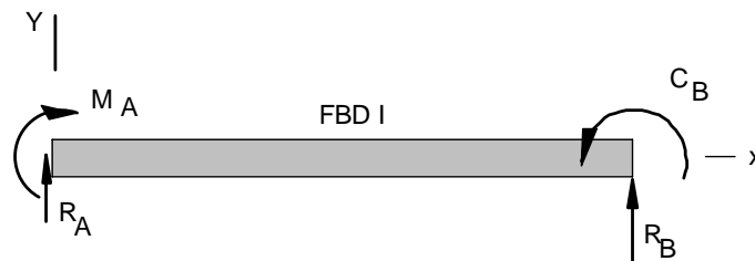
Figure 10. Free-body diagram of the propped cantilever beam.
