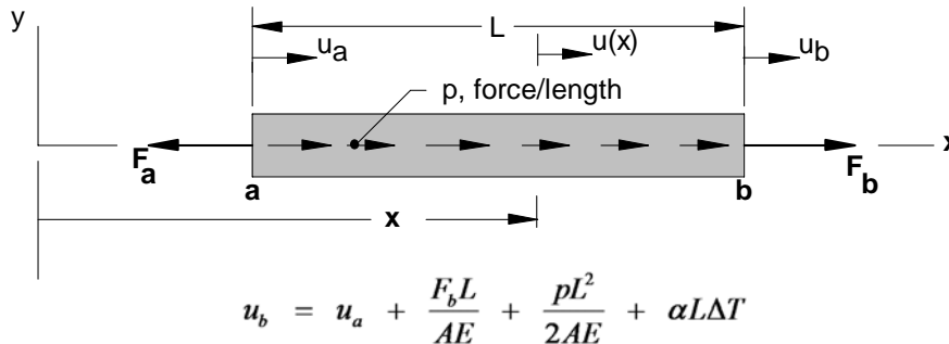
Figure 1. Material Law Formulas for a uniform bar with end centric axial and centric uniform distributed loads plus temperature change.
