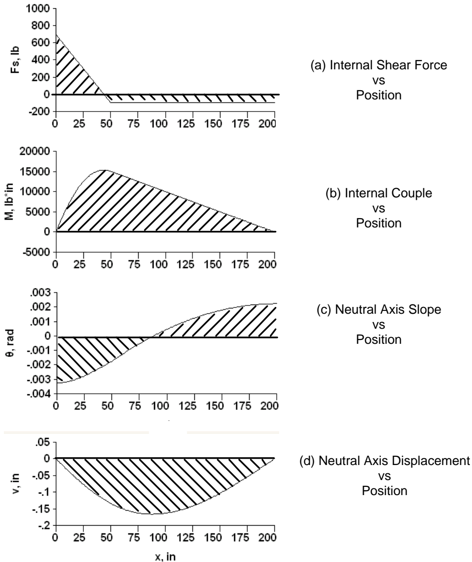
Figure 8. Shear, bending couple, slope and displacement diagrams for simply supported beam.
