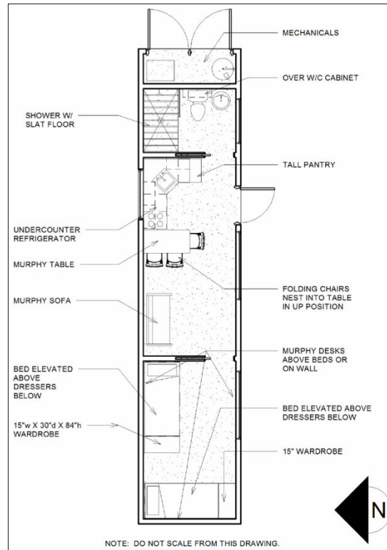
Figure 4: Floor Plan
