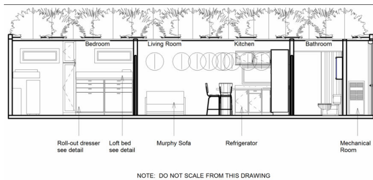
Figure 5: Building Section, South
