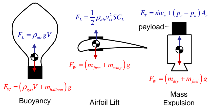
Fig.1 Three principles of powered flight – showing vertical forces only
