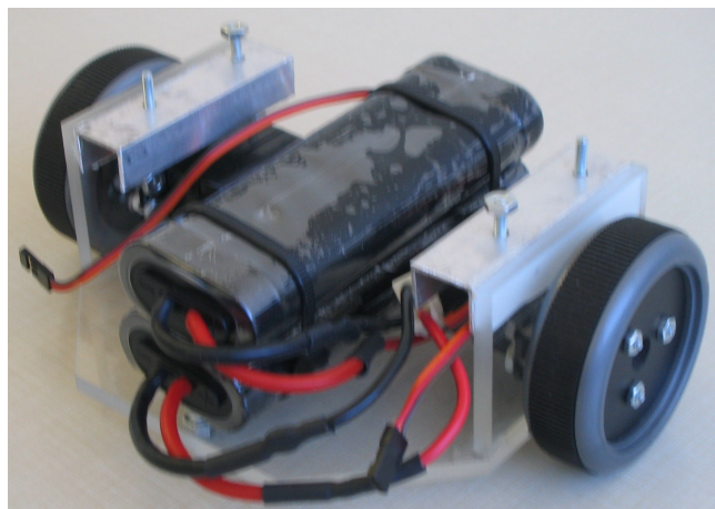
Figure 4: Bottom-plate
