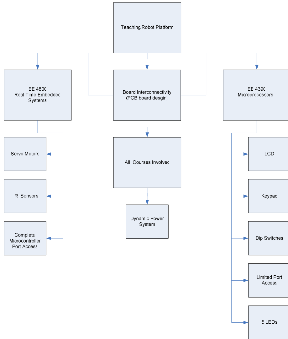
Figure 1: Project block diagram
