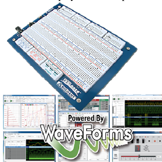
Fig. 1 Electronic Explorer Board
