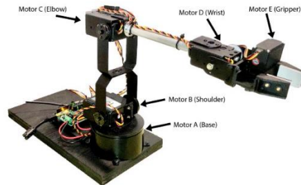
Figure 2 Robotic arm
